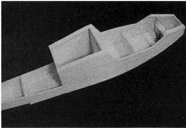
Triangle stock and bottom sheeting glued in place.
