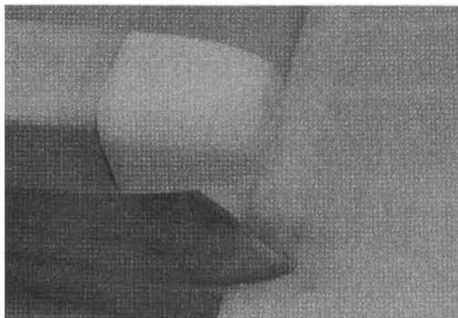
After fin was fiberglassed, foam block was glued to the firewall and shaped. Glass cloth was then laid over foam with epoxy to form cowl.
