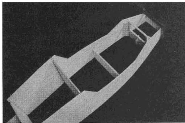
Front is pulled together using clamps. Note 5/32" i.d. brass tube is attached to F2 before installation.
