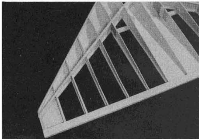
Center, tip and L/E sheeting added on bottom side. Blocks added to complete L/G mounts.
