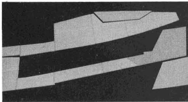
Fuselage sides cut out and fin doubler glued to them. Bulkhead placement lines marked on sides.
