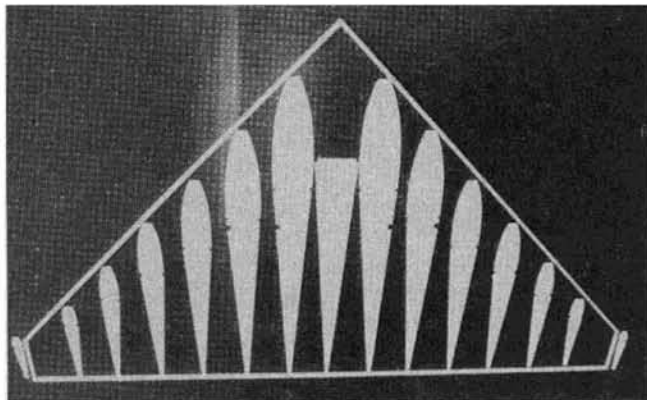
Layout of wing frame and all the ribs.
