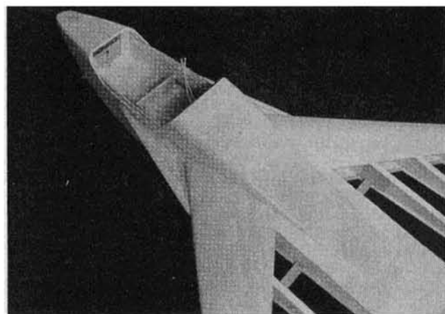
Wing root extensions added. Note NyRods protruding into cockpit area.
